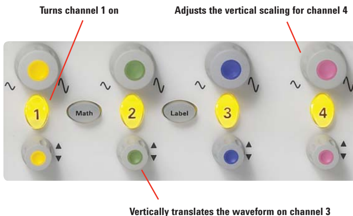
Figure 16. Front panel vertical control section on an Agilent InfiniiVision 5000 Series oscilloscope
