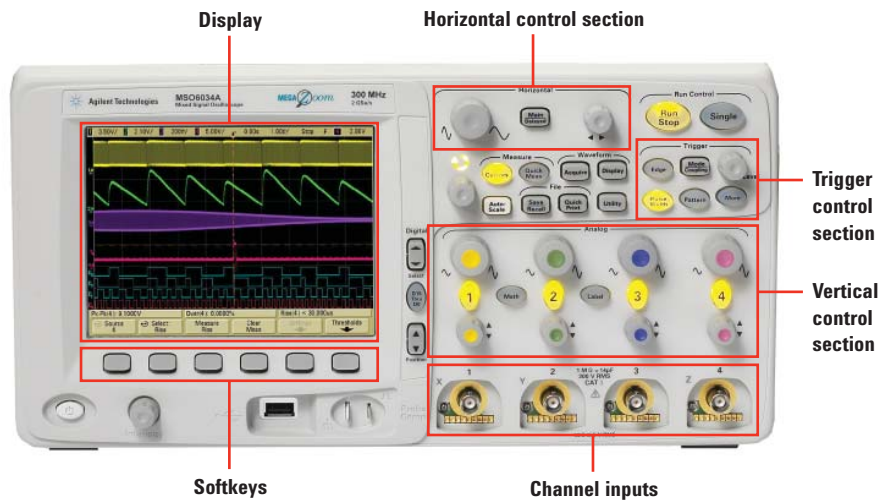
Figure 8. Front panel on the Agilent InfiniiVision 5000 Series oscilloscope
