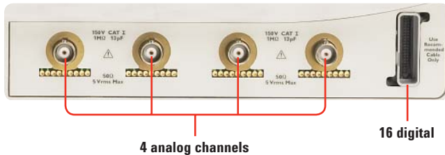
Figure 13. Front panel inputs for the four analog channels and 16 digital channels on a mixed-signal oscilloscope
